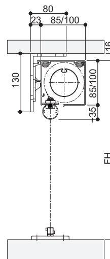
Installation with ceiling bracket
