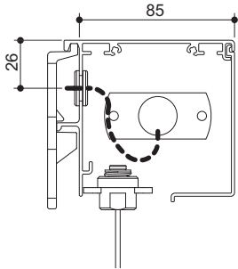
Box detail VW cable - cable exit towards the rear Q85
