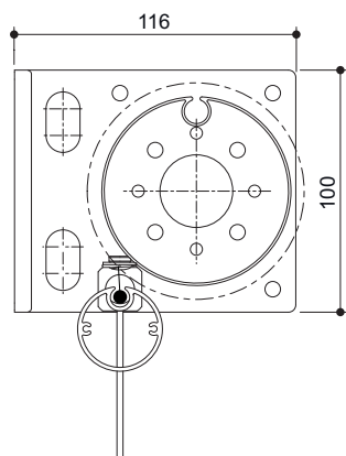
Wall installation
