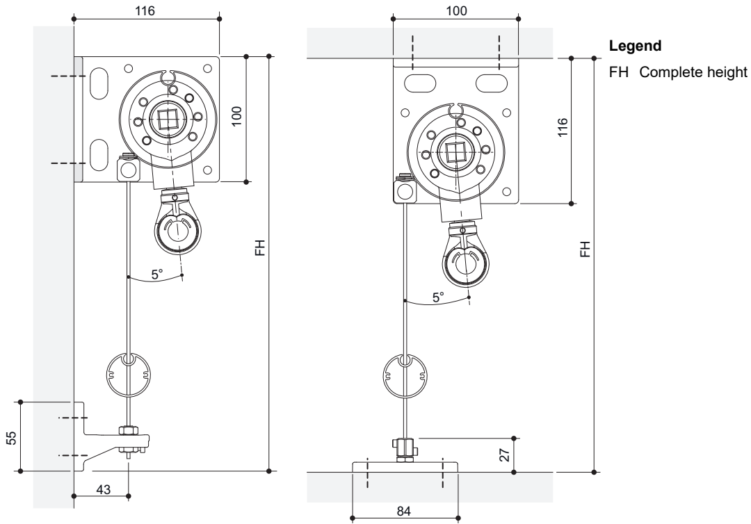
Installation of the bracket towards the back
