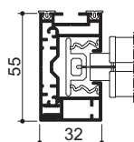
Single guide rail 32x55
