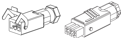
STAS 3 connector with bracket
