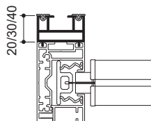
Adapter profile for guide rail spacing
