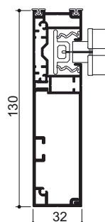
Deep guide rail 32x130
