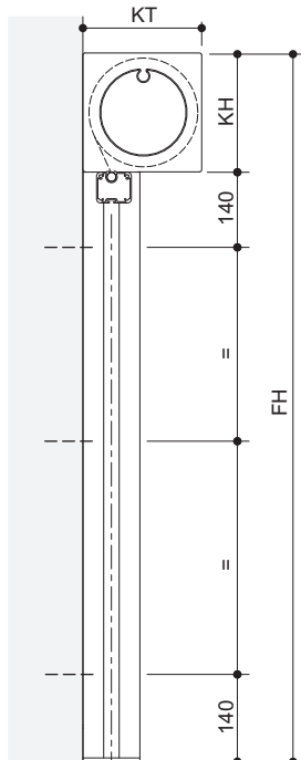
Direct installation - left roller
