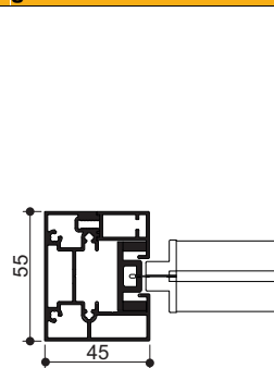
Fig. 5: Guide rail 55x45 mm
