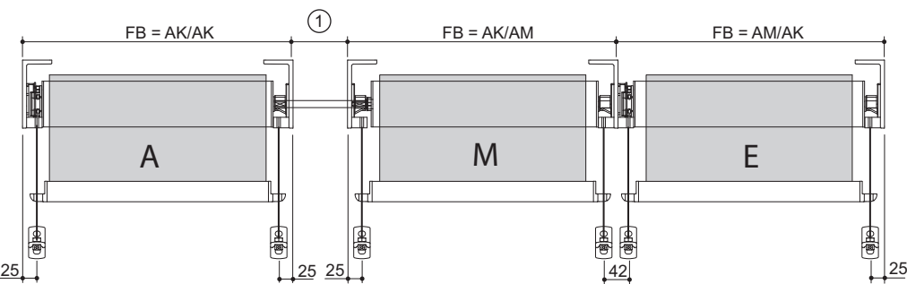
Combination in 3 parts with spacer - linked
