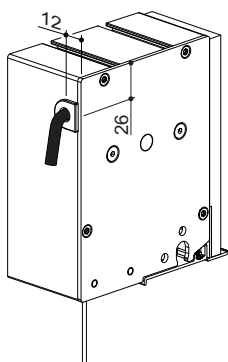
Cable exit towards the rear
