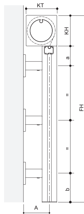
Installation with spacers - right roller (Not with crank handle drive)
