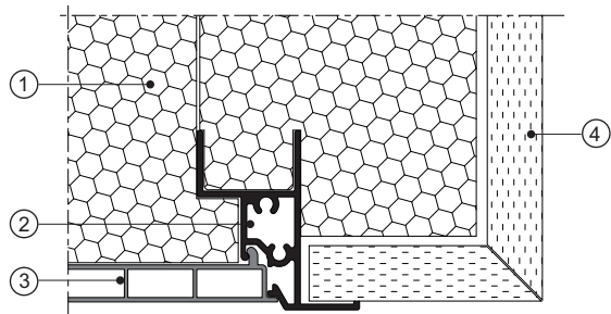
Lintel view from below on the inside Gypsum board
