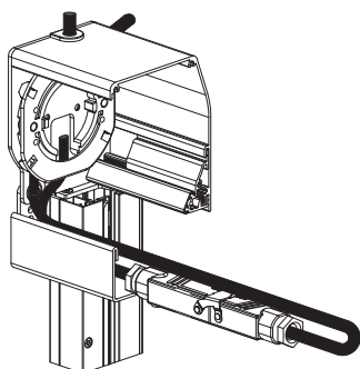
Hirschmann connector in the inspection cover
