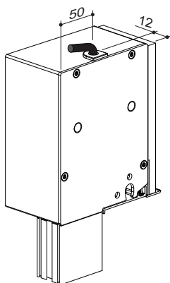
Cable exit towards the top
