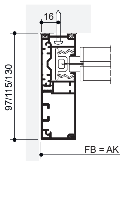
Direct installation with deep guide rail
