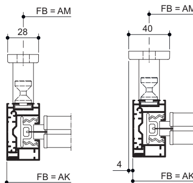
Guide rail spacers
