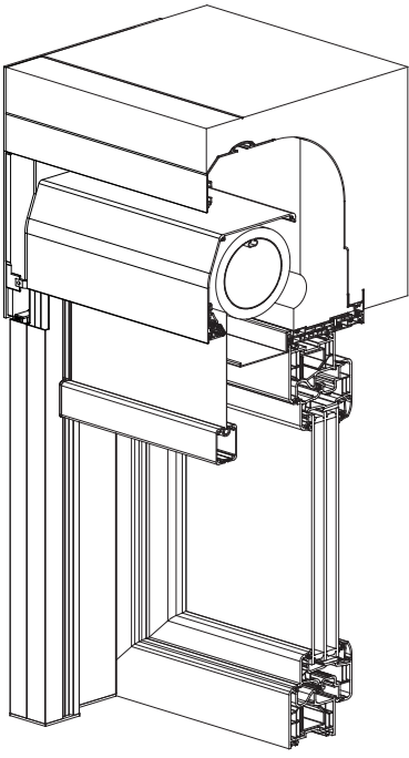
TOP FOAM screen protect .S without front skirt
