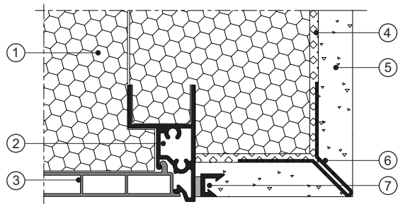
Lintel view from below on the inside Plaster (standard)
