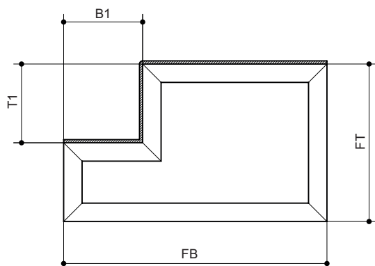
Special design 2C
