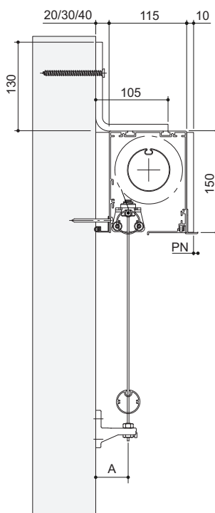
Installation with a mounting bracket
