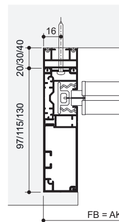
Direct installation with deep guide rail and insulation on the rear side
