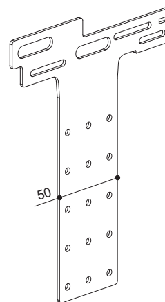
Fastening handle strengthened (optional)
