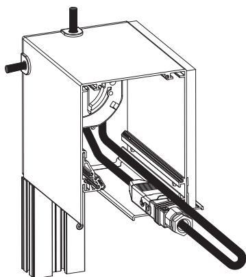
Hirschmann connector stored in the box and cable extension towards the outside
