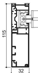
Deep guide rail 32x115
