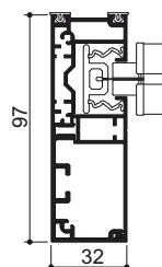
Deep guide rail 32x97
