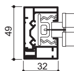
Adapter profile for guide rail spacing
