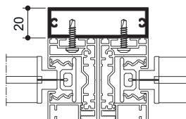
Adapter profile for post and beam installation - single
