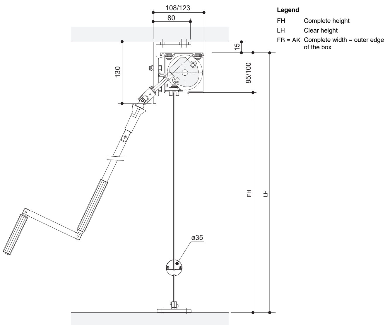
Design Crank handle drive with funnel at the rear side
