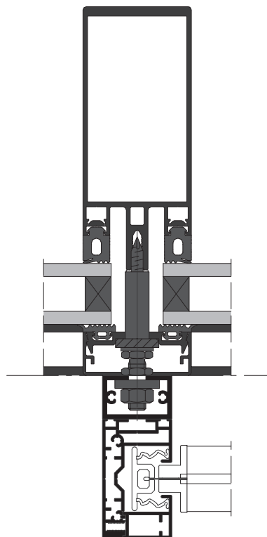
Adapter profile for post and beam installation - single
