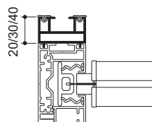
Adapter profile for guide rail spacing
