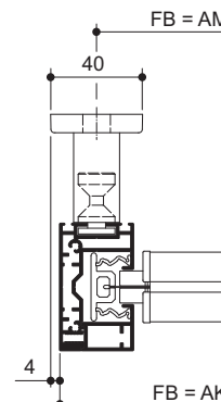
Guide rail spacer with large base plate
