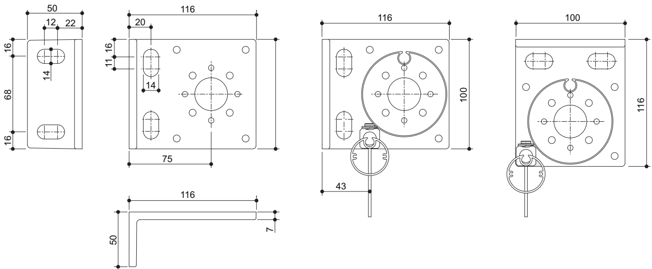
Installation of the bracket towards the back
