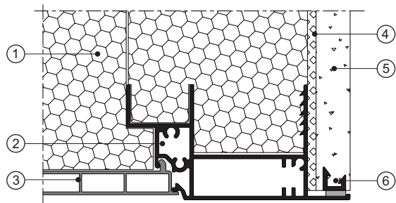
Lintel view from below on the inside Aluminium
