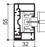
Adapter profile for guide rail spacing
