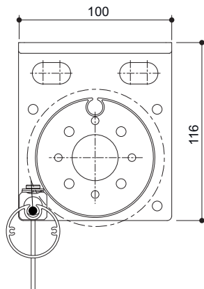
Ceiling installation
