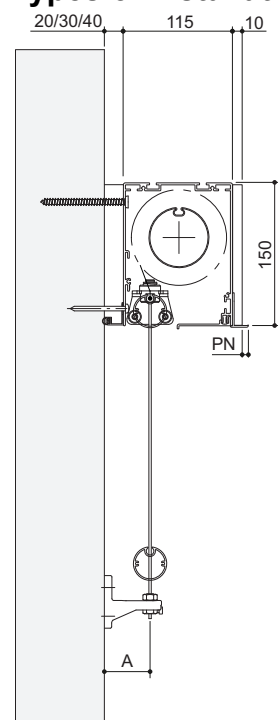
Installation directly through the box
