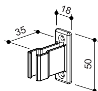
Crank holder 35 mm
