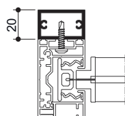
Adapter profile for post and beam installation - single
