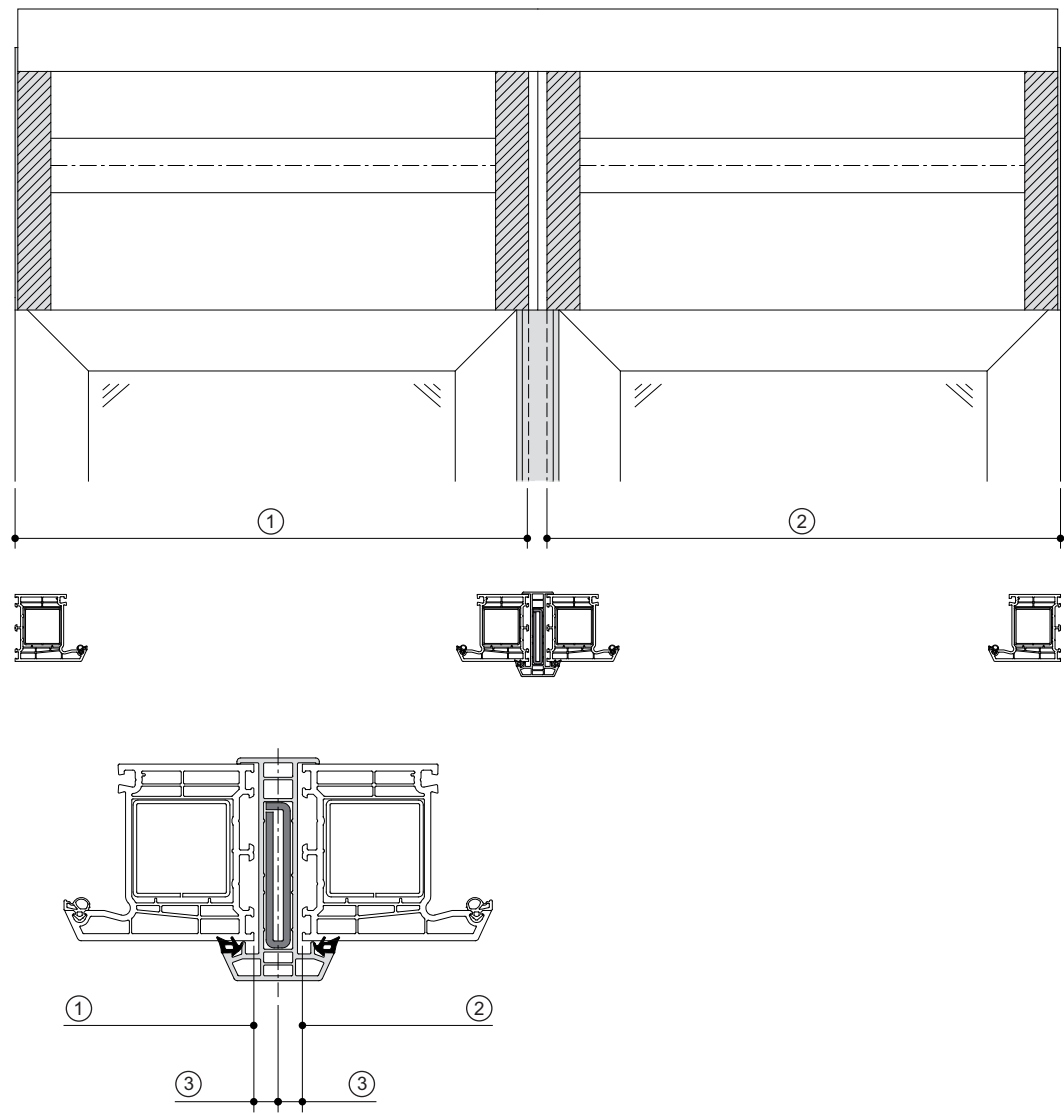
View: Detail with statics linkage element and steel insert
