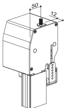
Cable exit towards the top
