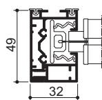
Single guide rail 32x49
