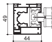
Single guide rail 44x49 Crank drive
