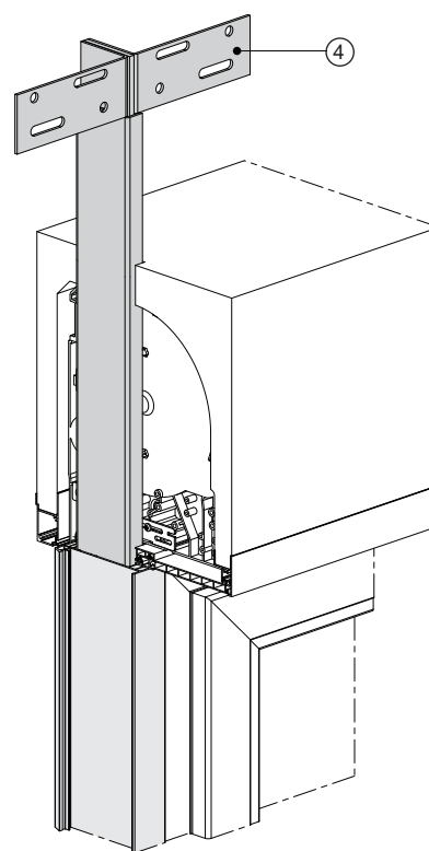
View: Detail with box connection to the brickwork
