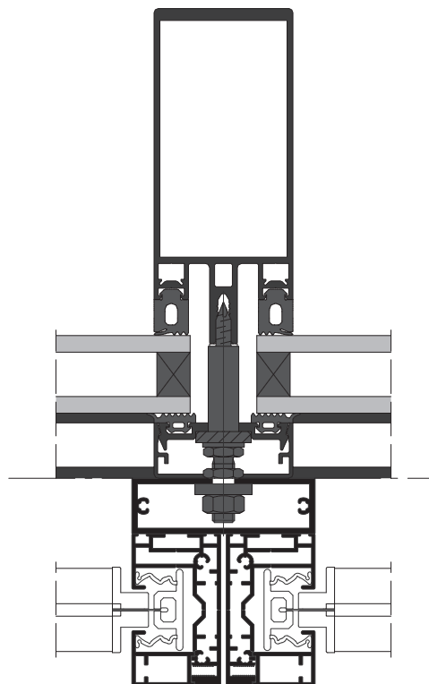
Adapter profile for post and beam installation - double
