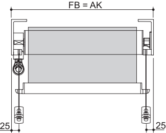
Single unit with crank handle drive
