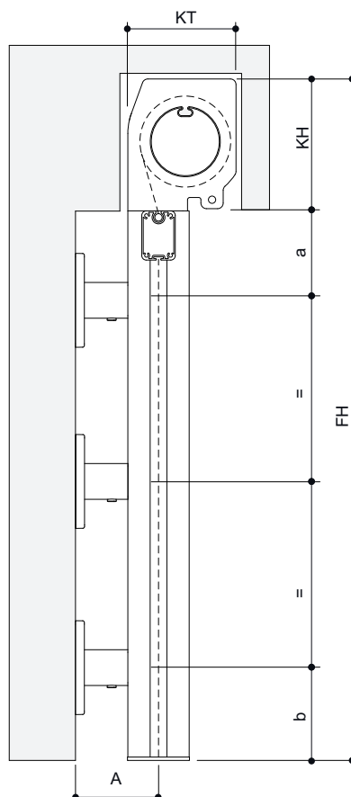
Installation with spacers
